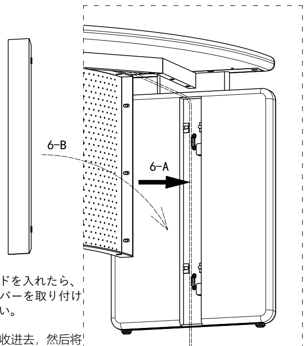
First, retract the wires and then install this board back in place
